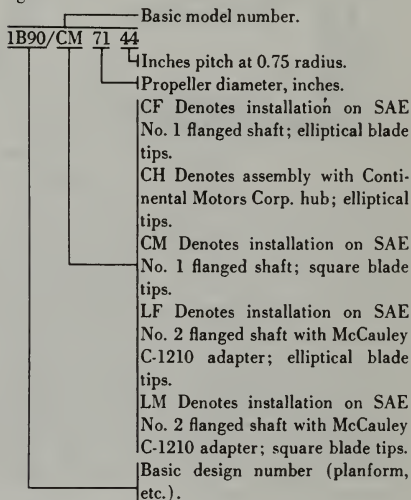
FIGURE 7-10. Complete propeller model number.
